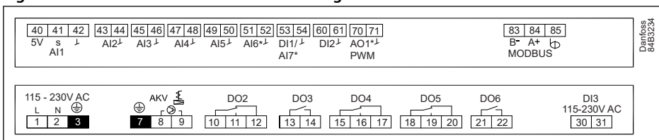
Figure 16: Electrical connections AK-CC55 Single Coil
