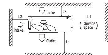
Minimum installation space
