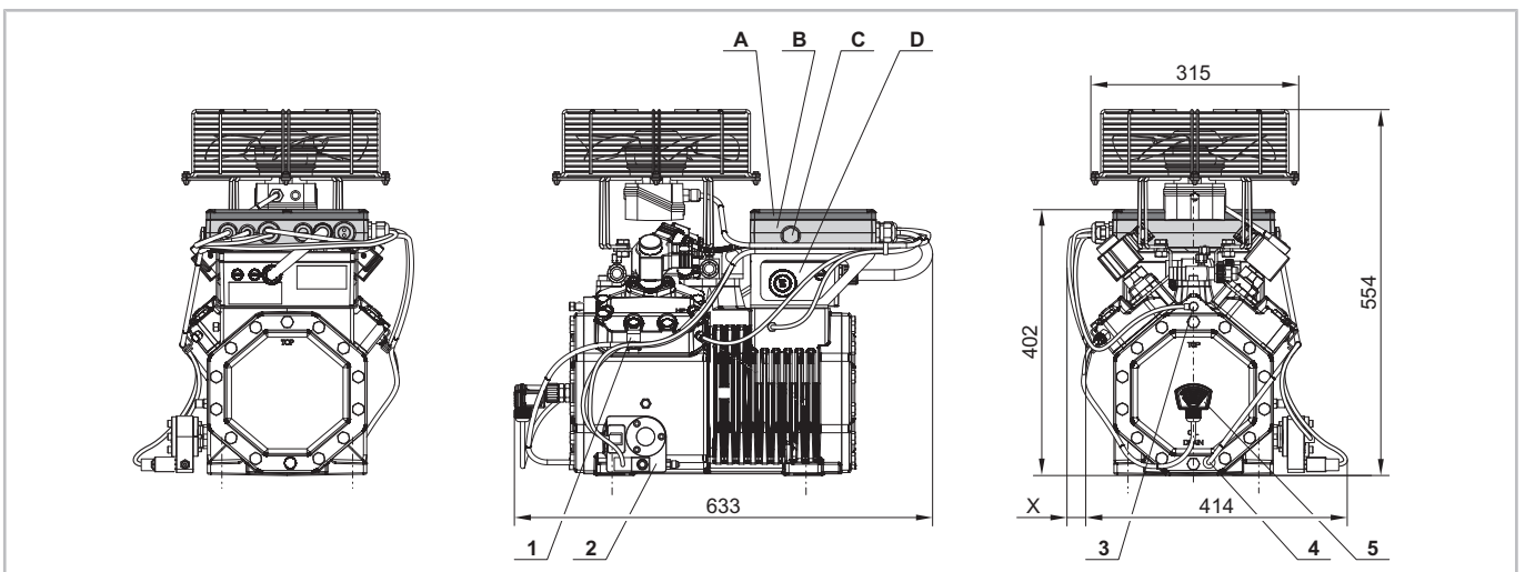
Fig. 4: 4FES-3(Y) .. 4BES-9(Y) and 4FESH-3Y .. 4BESH-9Y with all options offered by CM-RC-01.
