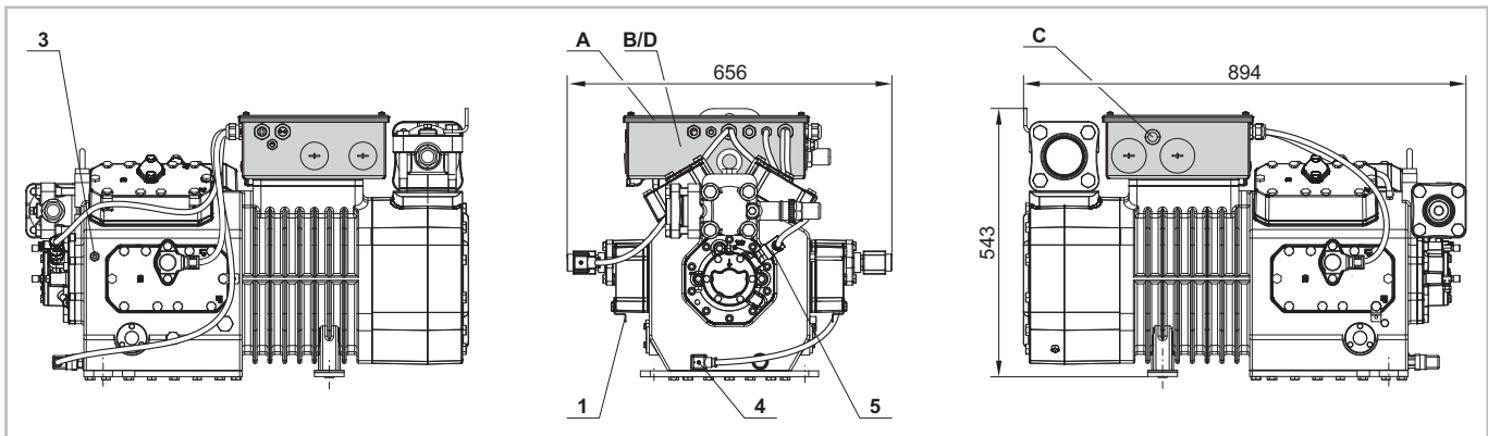
Fig. 6: 8GE-50(Y) .. 8FE-70(Y) with all options offered by CM-RC-01. The cables of the pressure transmitters are not shown.
