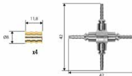
Cross Fitting
