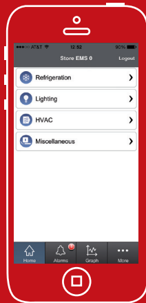
Application access
