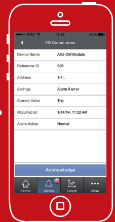
Alarm details
