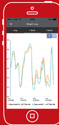
Device graphs
