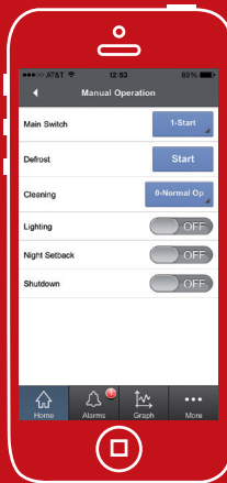
Device overview
