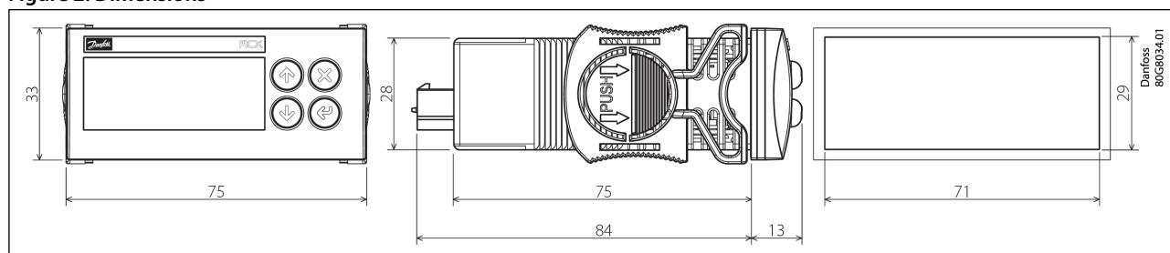
Figure 2: Dimensions
