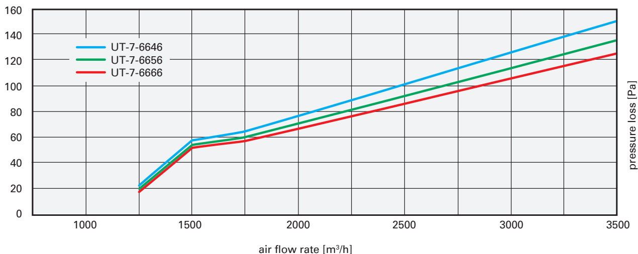
Loss of pressure as a function of air flow rate for the filters
