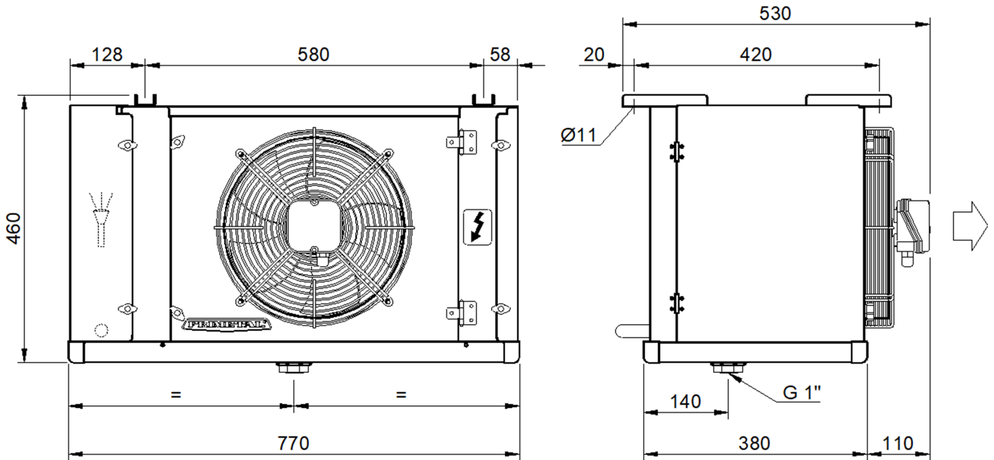
DIRECT EXPANSION EVAPORATOR - FRM-165
